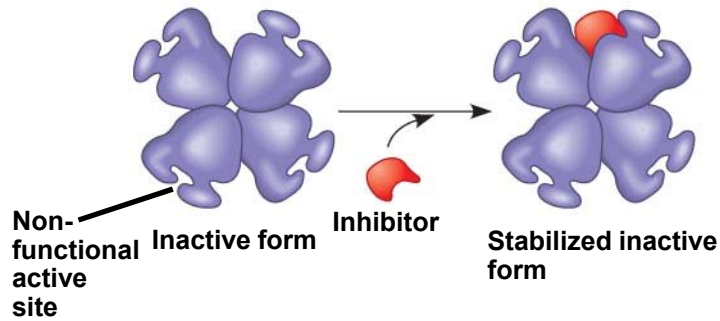
(a) Allosteric activators and inhibitors
