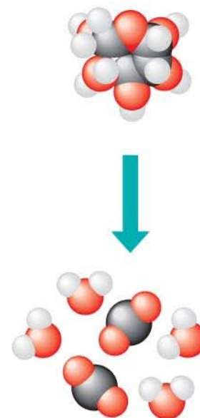
(c) Chemical reaction
